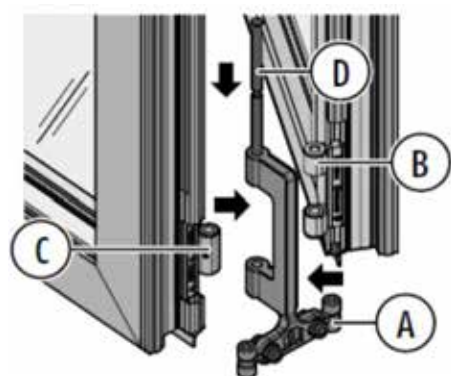
Photo 9 Bottom bracket assembly A: Bottom running bracket B: Female part of hinge. C: Male part of hinge. D: Long hinge pin.
