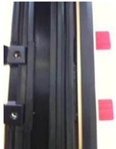
Photo 6 Gasket covers pre-drilled fixing location and screw once fitted
