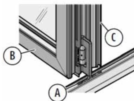
Photo 10 Bottom bracket fully assembled
