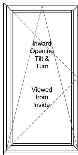
Tilt & Turn Opening Jamb Inc 30mm Add-On
