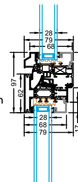
Tilt & Turn Fixed Mullion
