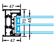
45mm Glass Unit
