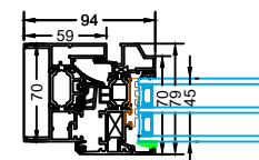
45mm Glass Unit
