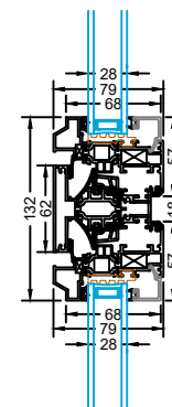
Tilt & Turn Transom
