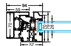
32mm Glass Unit
