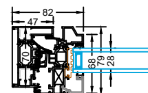
28mm Glass Unit
