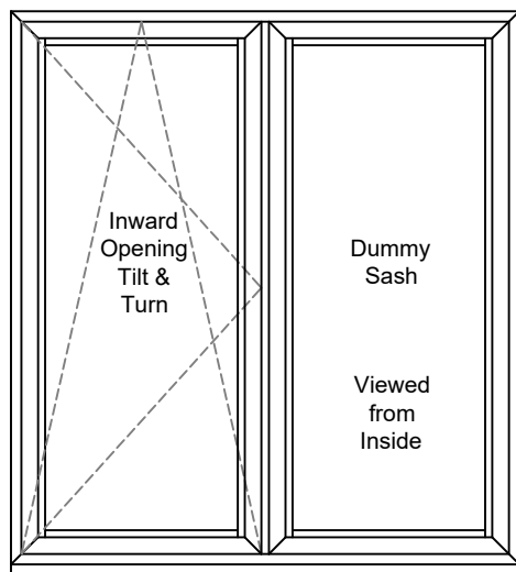
Tilt & Turn Mullion
