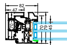
45mm Glass Unit
