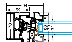
32mm Glass Unit
