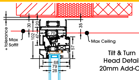
Tilt & Turn Head Detail No Trickle Vent
