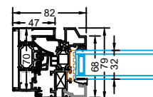
32mm Glass Unit
