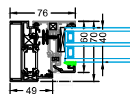
40mm Glass Unit
