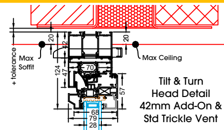
Tilt & Turn Head Detail 20mm Add-On
