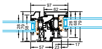
Tilt & Turn Fixed Mullion
